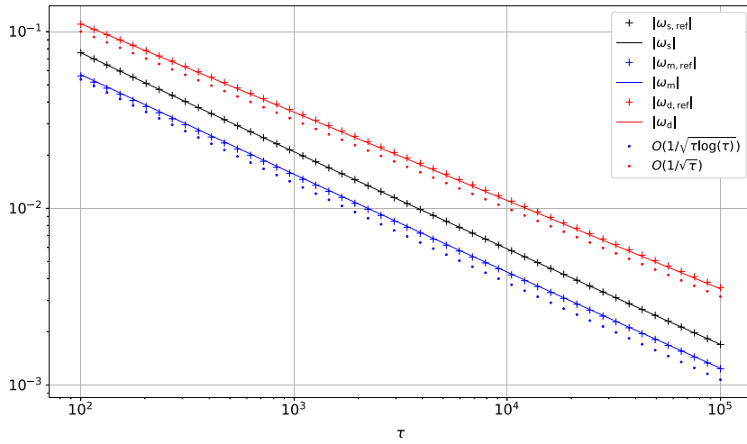
FIGURE 1 The asymptotic resonances \omega_s (single particle), \omega_m (monopole), and \omega_d (dipole) given by the formulas in Propositions B.1 and Corollary 3.3 and the corresponding resonances obtained using reference solutions [Colour figure can be viewed at wileyonlinelibrary.com]
